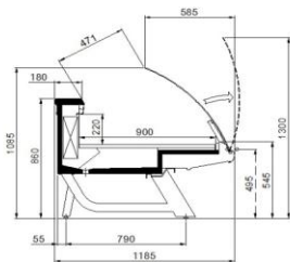
Piedi verniciati tub. Prepainted tube legs
